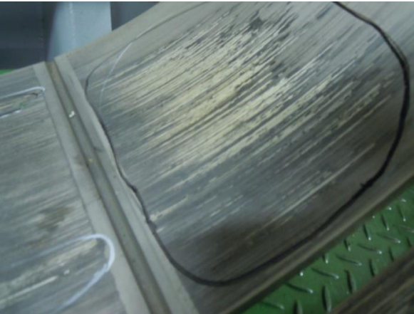
Breakdown analysis Investigation and Supervision during crosshead bearing shell replacement for MAN-B&W 9K90MC-C, (Hong-Kong)
